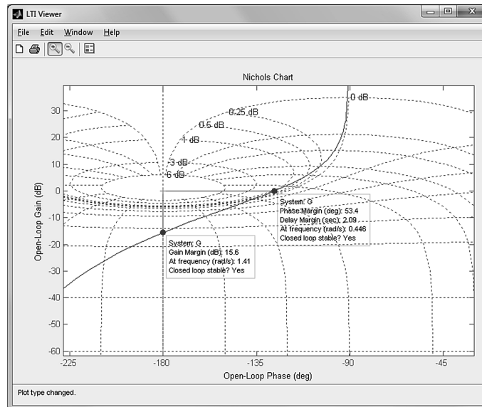
FIGURE E.5 LTI Viewer used for Nichols chart: a. M-file; b. LTI Viewer
