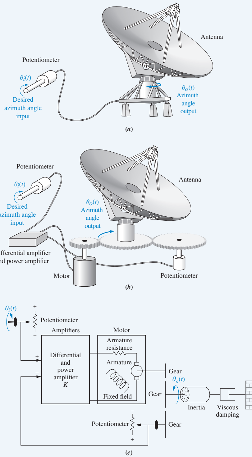
FIGURE 1.8 Antenna azimuth position control system: a. system concept; b. detailed layout; c. schematic (figure continues)
