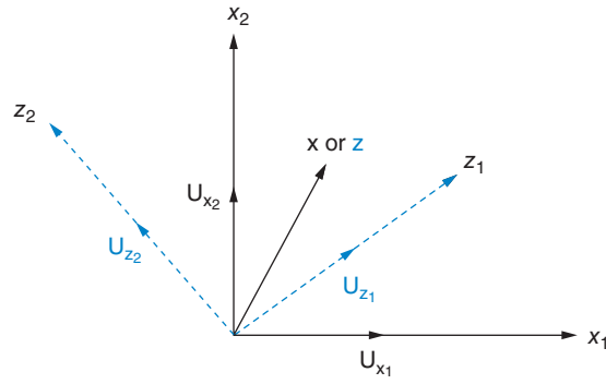
FIGURE L.1 State-space transformations
