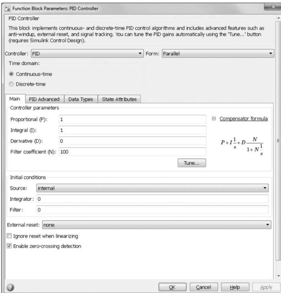
FIGURE C.20 Function Block Parameters window for the PID controller
