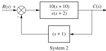
FIGURE P7.17 Closed-loop systems with nonunity feedback
