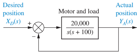
FIGURE P13.9 Simplified block diagram of a floppy disk drive
