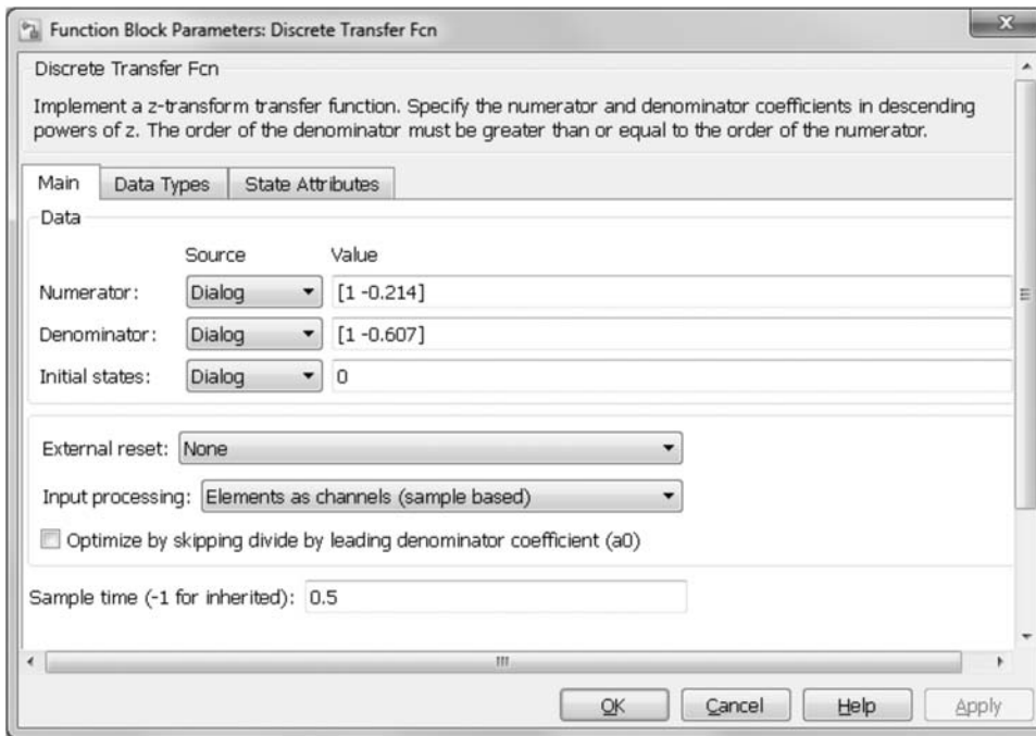
FIGURE C.17 (Continued) b. Discrete Transfer Fcn block
